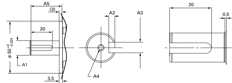
Shaft detail
